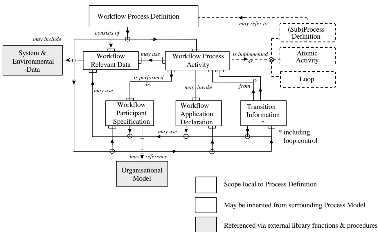
Figure 3-1: Meta-Model top level entities
