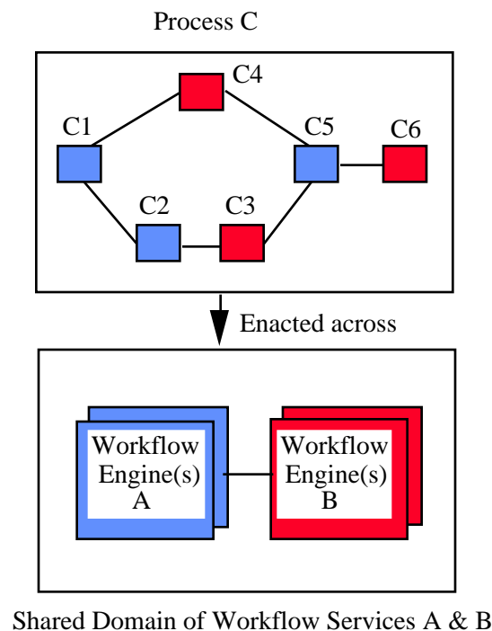
Fig 15 - Peer-Peer Model
