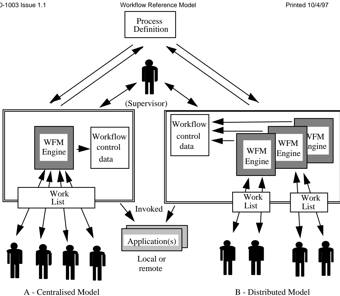
Figure 4 - Standard workflow enactment service boundary
