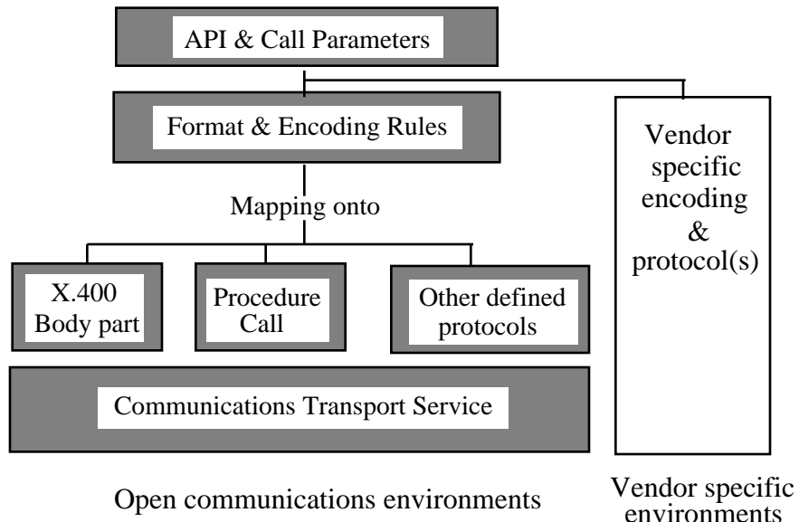
Fig 20 - WAPI protocol support
