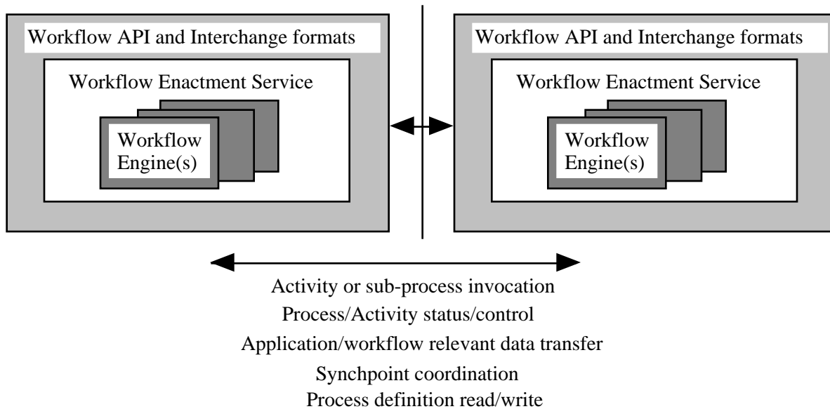
Figure 17 - Workflow interoperability interface
