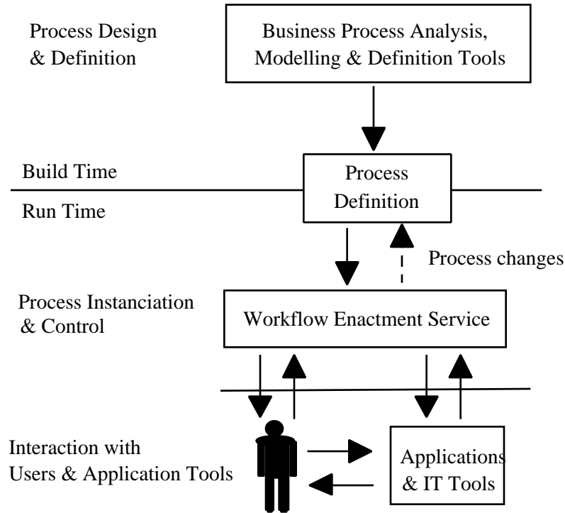
Figure 1- Workflow System Characteristics
