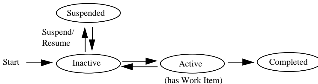
Figure 8 - Example state transitions for an activity instance
